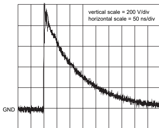
unclamped +1 kV ESD voltage waveform (IEC61000-4-2 network)
